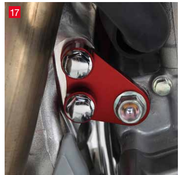
17 Front Engine Hanger (CRF450R & CRF250R only)
