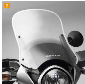
2 Tall Windshield A polycarbonate windshield that is 170mm higher than the standard version and features deflectors for improved protection and rider comfort.
